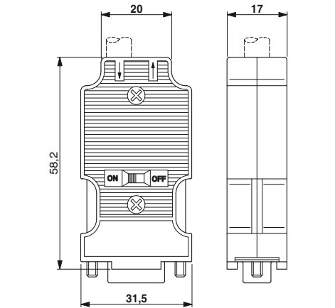
Dimensional drawing SUBCON-PLUS-.../AX...
