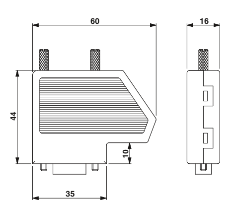
Dimensional drawing SUBCON-PLUS...
