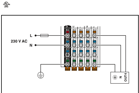
4 outputs, 12 ... 253 V AC wide range
