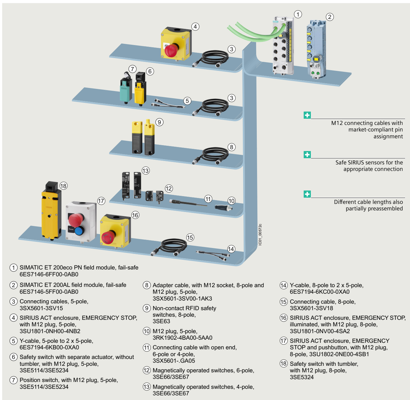
Safety field system composed of SIRIUS sensors and SIMATIC ET 200 with the M12 connection method
