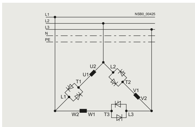
Inside-delta circuit: Rated current I_e corresponds to approx. 58% of the rated motor current I_n , six cables to the motor (as for star-delta (wye-delta) starters)
