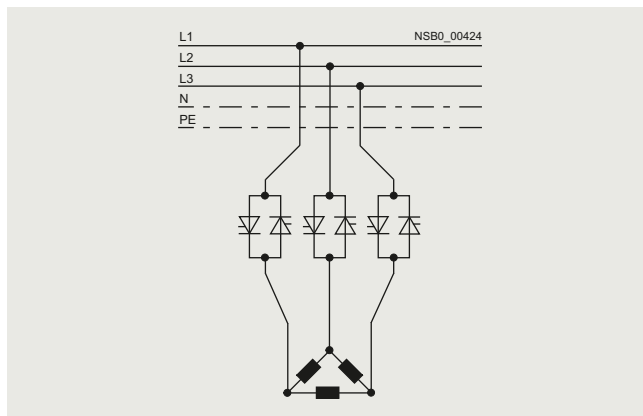
Standard (inline) circuit: Rated current I_e corresponds to the rated motor current I_n , three cables to the motor
