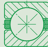
Axial-Ball thrust bearing PBAD 12,7 x 12,7
