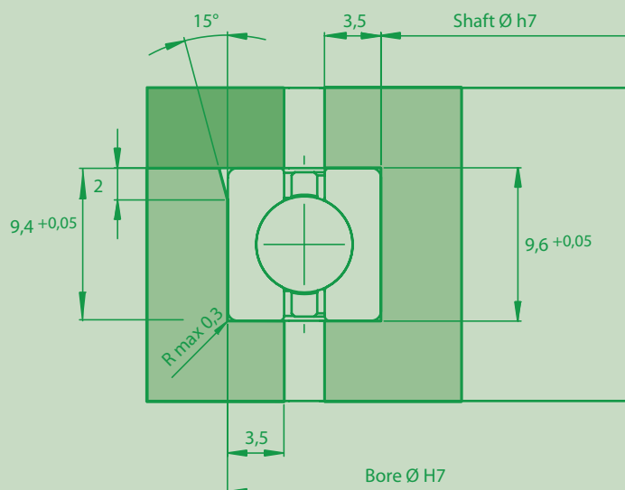
Fitted dimensions
