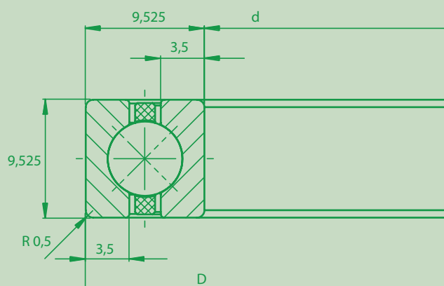
Bearing dimensions
