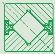
Axial-angular roller bearing PSA-08 8 x 8 mm
