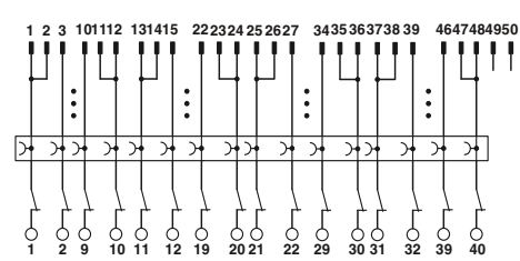
Connection scheme FLKM 50/KDS3-MT/PPA/S7-300
