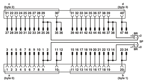
Connection scheme for FLKM 50-PA/.../DIO/S7-1,500
