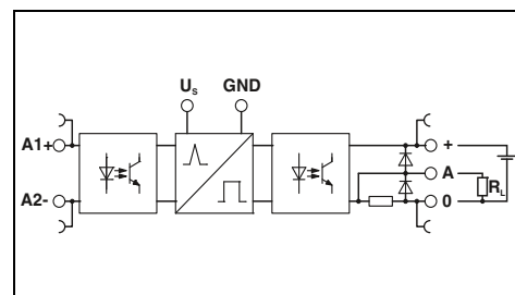
Solid-state relay module for the extension of input pulses, DC output max. 100 mA
