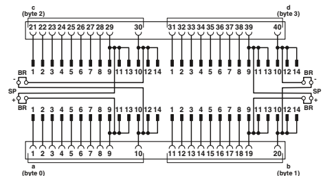
Connection scheme for FLKM 4X14-PA/.../DIO/S7-1,500
