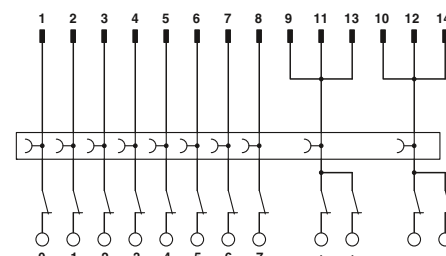
Connection scheme FLKM 14/KDS3-MT/PPA/PLC
