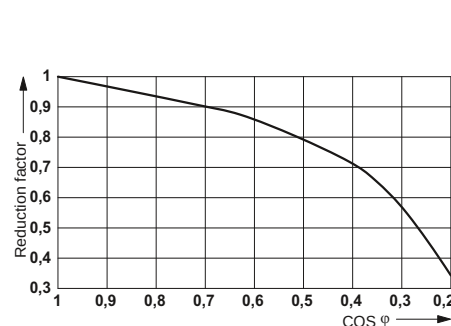
Service life reduction factor with various cos phi
