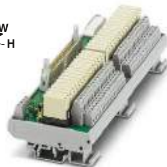
Output module with 32 miniature relays, 1 N/O contact
