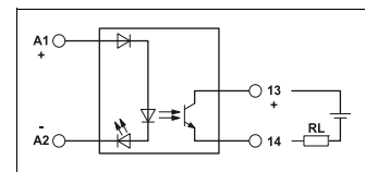
Figure 3: 2-conductor output
