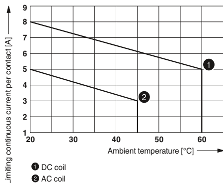
Contact derating
