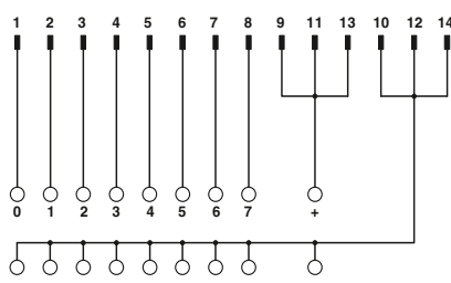
Connection scheme VIP-2/.../FLK14/8M/PLC
