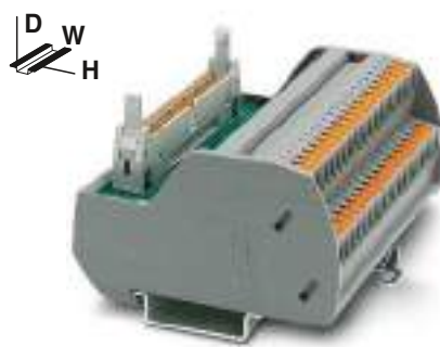
Passive interface modules for SIMATIC® S7-400 with Push-in connection
