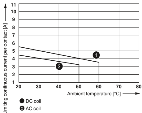
Contact derating
