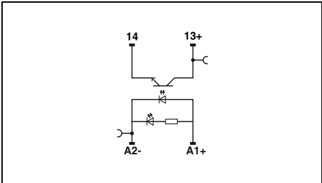
Solid-state relay module with Push-in connection, DC output max. 3 A
