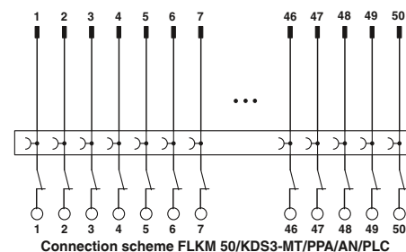
Connection scheme FLKM 50/KDS3-MT/PPA/AN/PLC
