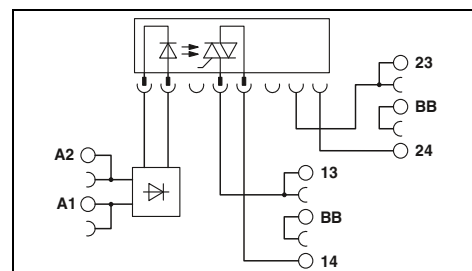
Solid-state relay module with additional floating terminal point, AC output max. 2 A
