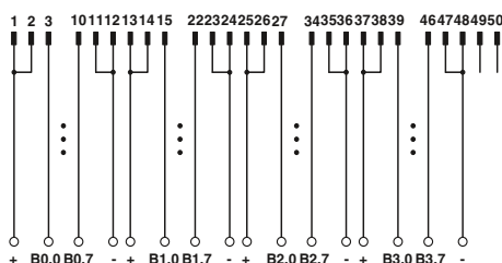
Connection scheme VIP-2/SC/FLK50/PLC
