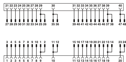
Connection scheme FLKM 50-PA/AN/S7-1,500
