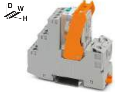
2-changeover-contact industrial relay module with screw connection and manual operation
