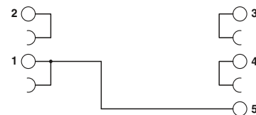
Connection scheme PLC-VT/ACT
