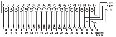
Connection scheme: FLKM-PA-D37/ETHA
