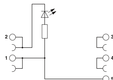
Connection scheme PLC-VT/ACT/LA
