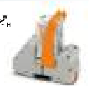
2-changeover-contact octal relay module with Push-in connection and manual operation
