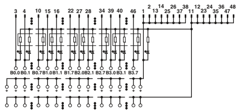
Connection scheme FLKMS 50/32IM/LA/PLC
