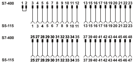
Connection scheme: FLKM S115/S400/SO155
