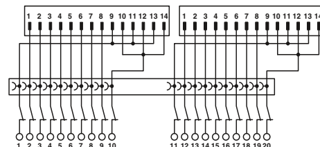
Connection scheme FLKM-2FLK14/KDS3-MT/PPA/S7
