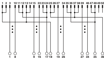
Connection scheme VIP-2/.../FLK50/AB-1756
