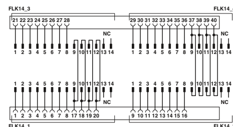
Connection scheme FLKM 4X14-PA/AN/S7-1,500
