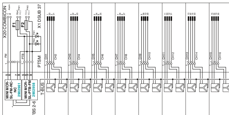
TC-D37SUB-ADIO16-M-P-P-UNI and TC-D37SUB-AIO16-M-PS-UNI connection scheme
