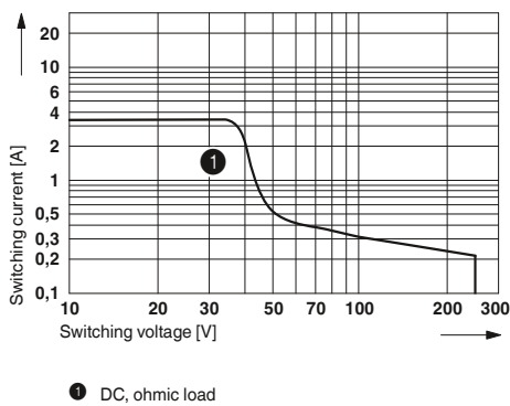
Interrupting rating
