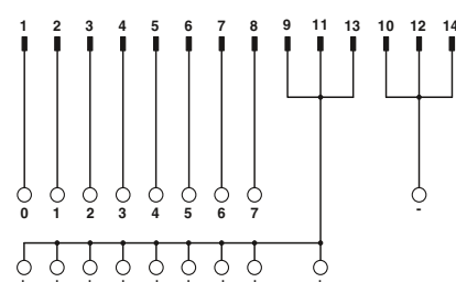
Connection scheme VIP-2/.../FLK14/8P/PLC
