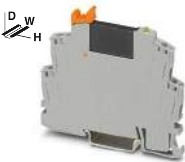
Solid-state relay module with screw connection, DC output max. 3 A
