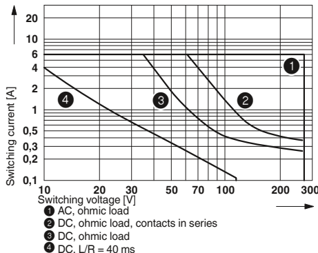
Electrical interrupting rating for PLC...24DC/1-1/ACT? with 2 N/O relays
