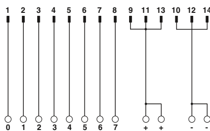
Connection scheme VIP-2/SC/FLK14/PLC
