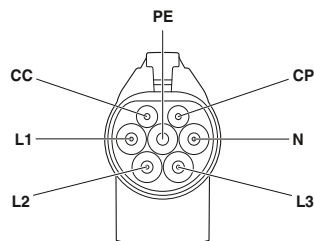
GB/T vehicle charging connector pin assignment
