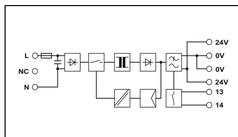
Power supply 1 AC, 24 DC, 1.5 A DIN rail connector optional
