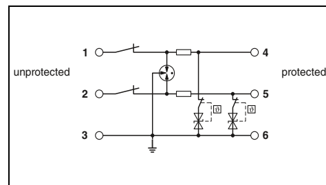
2-conductor with common reference potential, 3/6 connection grounded directly, with knife disconnection, e.g., for binary signals
