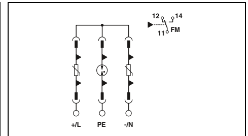
3-conductor system, DC+, DC-, PE for 220 V DC and 380 V DC, free of leakage current
