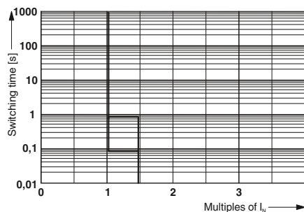
Tripping characteristic
