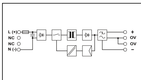
Power supply, 1 AC, \pm 15 V DC, 1 A NEC Class 2
