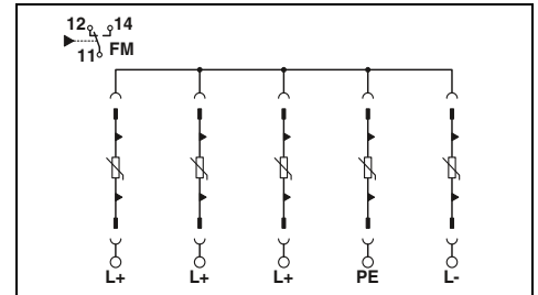
Pluggable surge protection, for PV applications up to 1000 V DC, 3 MPP trackers
