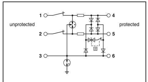
3-conductor with common reference potential, 3/6 connection grounded via gas-filled surge arrester, pluggable
