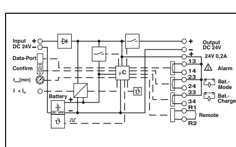
Uninterruptible power supply with integrated energy storage, 24 V DC / 24 V DC, 5 A, 1.3 Ah
