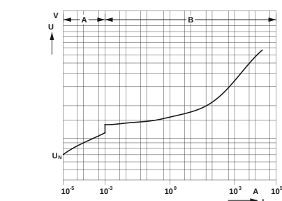
U/I characteristic curve of metal oxide varistors
