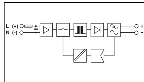
Power supply, 1 AC, 5 V DC, 2 A NEC Class 2
