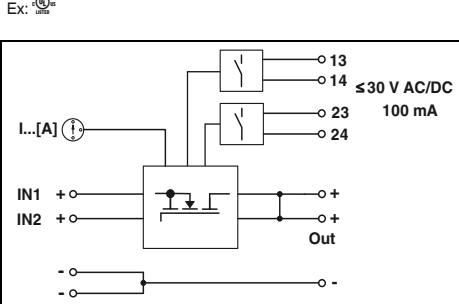
Active redundancy module 24 V DC, 2 x 40 A, 1 x 80 A
