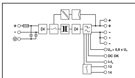
DC/DC converter, with protective coating, 96 - 110 V DC/24 V DC, 10 A
