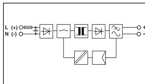
Power supply, 48 V AC, 24 V DC, 0.5 A NEC Class 2
