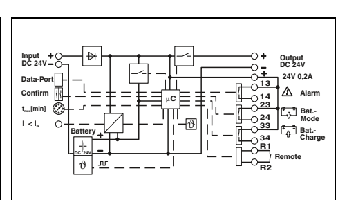
Uninterruptible power supply with integrated energy storage, 24 V DC / 24 V DC, 10 A, 3.4 Ah
