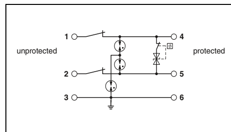
2-conductor, floating, pluggable, with knife disconnection, e.g., for actuator circuits
