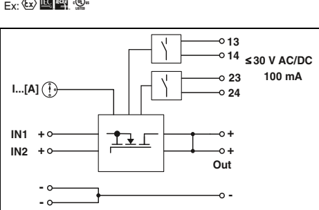
Active redundancy module, with protective coating, 24 V DC, 2 x 20 A, 1 x 40 A
