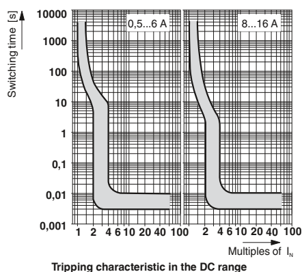
Tripping characteristic in the DC range
