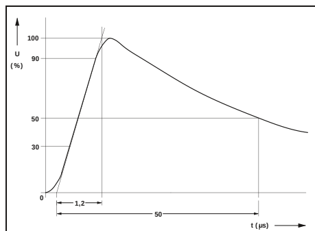
1.2/50 \mu s surge voltage pulse in acc. with IEC 60060-1
