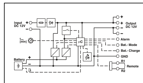
Uninterruptible power supply with integrated battery module, 12 V DC/12 V DC, 4 A, 46WH
