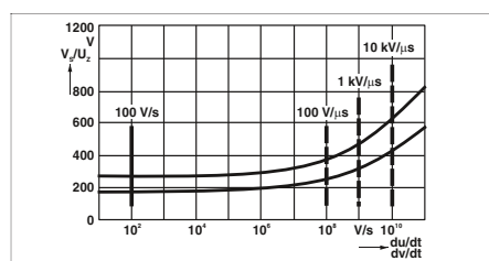
Ignition curve of a gas discharge tube — Static response behavior - - - Dynamic response behavior
