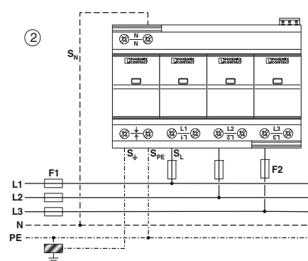
Application example ② Type 1 surge protective device for protecting three-phase TN/TT systems with 5 conductors; connected in branch wiring
