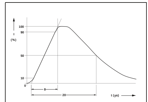
8/20 \mu\text{s} surge current pulse in acc. with IEC 60060-1
