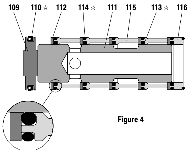
MAJOR VALVE CROSS SECTION DETAIL
